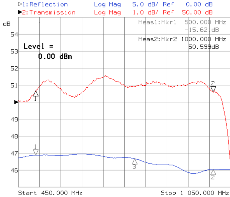
Frequency Response Curve @ 100 Watts Output
