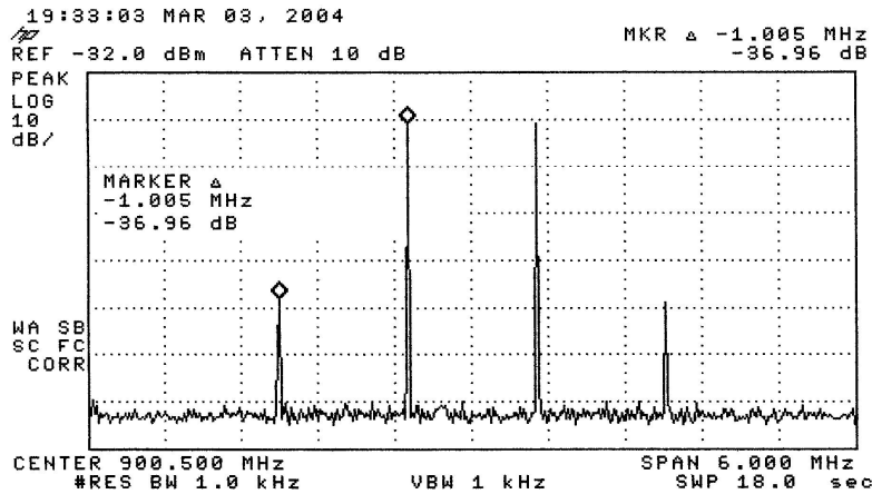
Two Tones 100 mwatts Avg. Per Tone @ 900 & 901MHz IP3 = +38dBm
